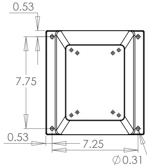
MOUNTING PATTERN
